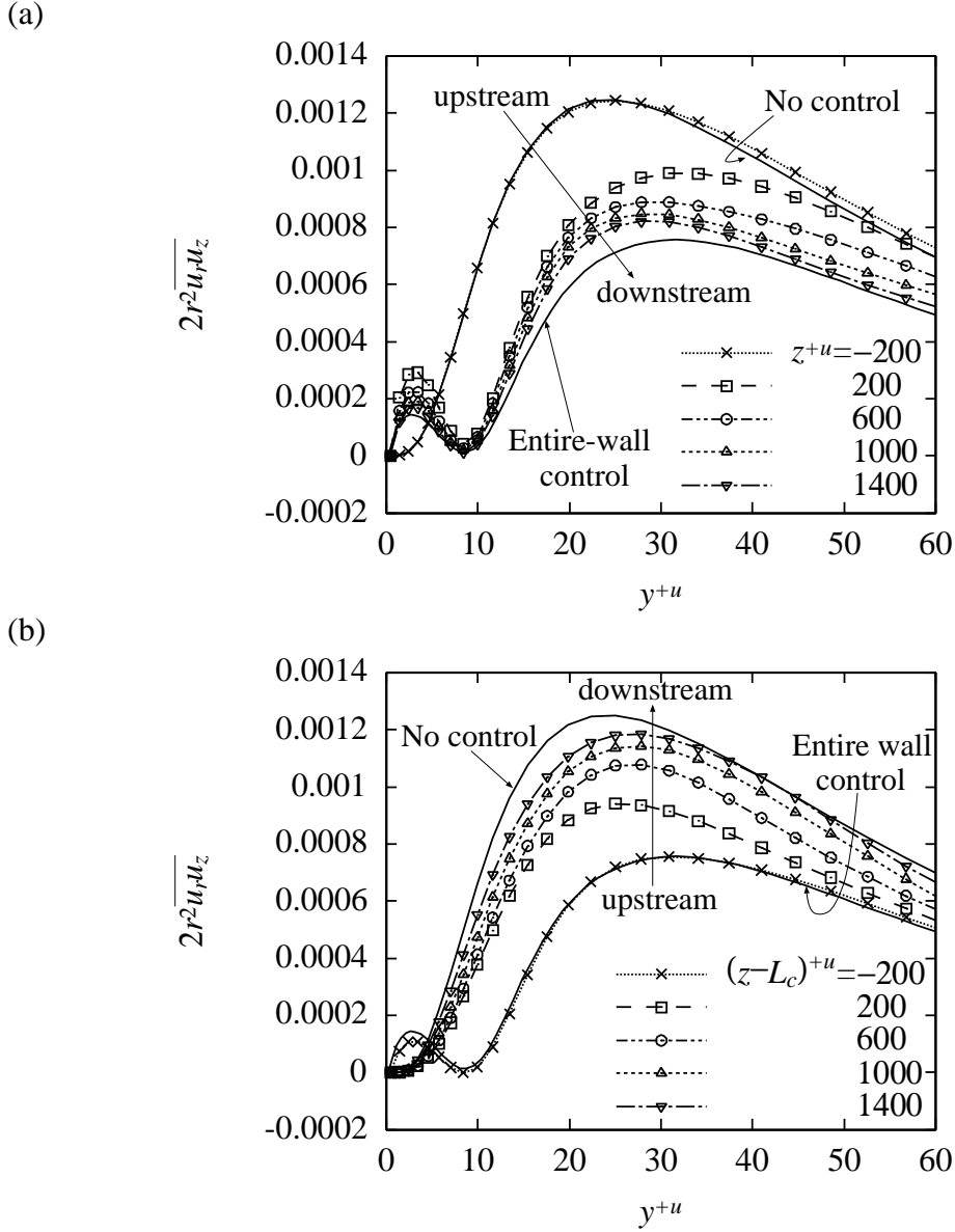
Fig. 9. Weighted Reynolds stress distribution at different streamwise locations (Case 4, L_c^{+u} = 7360 , y_d^{+u} = 15 ): (a) controlled region; (b) uncontrolled region.
