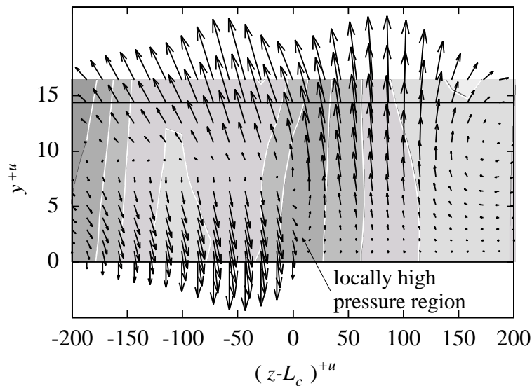
Fig. 11. Fluctuating velocity vector ( \vec{u}' ) and pressure (light gray, (p')^{+u} < -1.5 , to dark gray (p')^{+u} > 1.5 with increment of 0.5) around the end point of control projected to an r-z plane (Case 4, L_c^{+u} = 7360 , y_d^{+u} = 15 ): (a) in a region where the control ends with blowing ; (b) the same with suction. The coordinates and the vectors are stretched (10 times) in the wall-normal direction.
