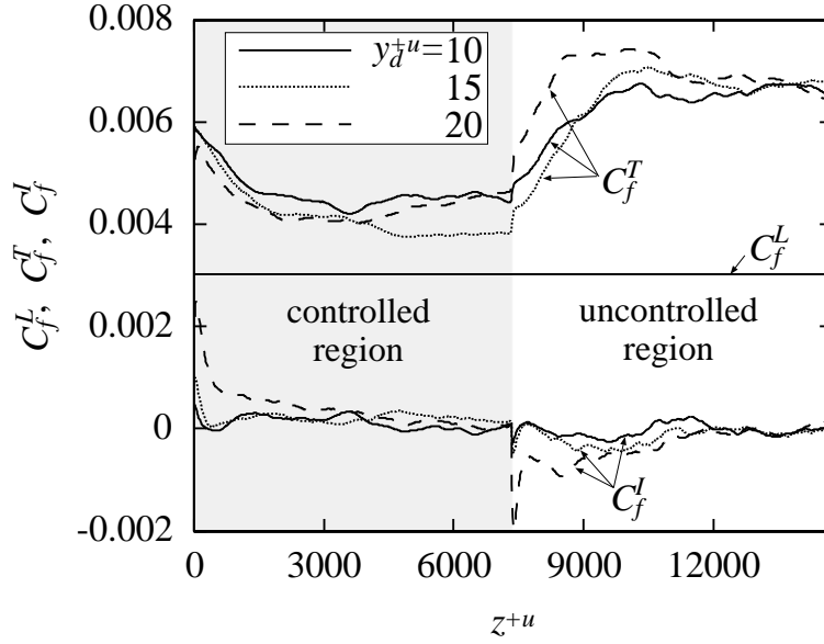
Fig. 8. Componential contributions to C_f(z) (Case 4, L_z^+ = 7360 ).
