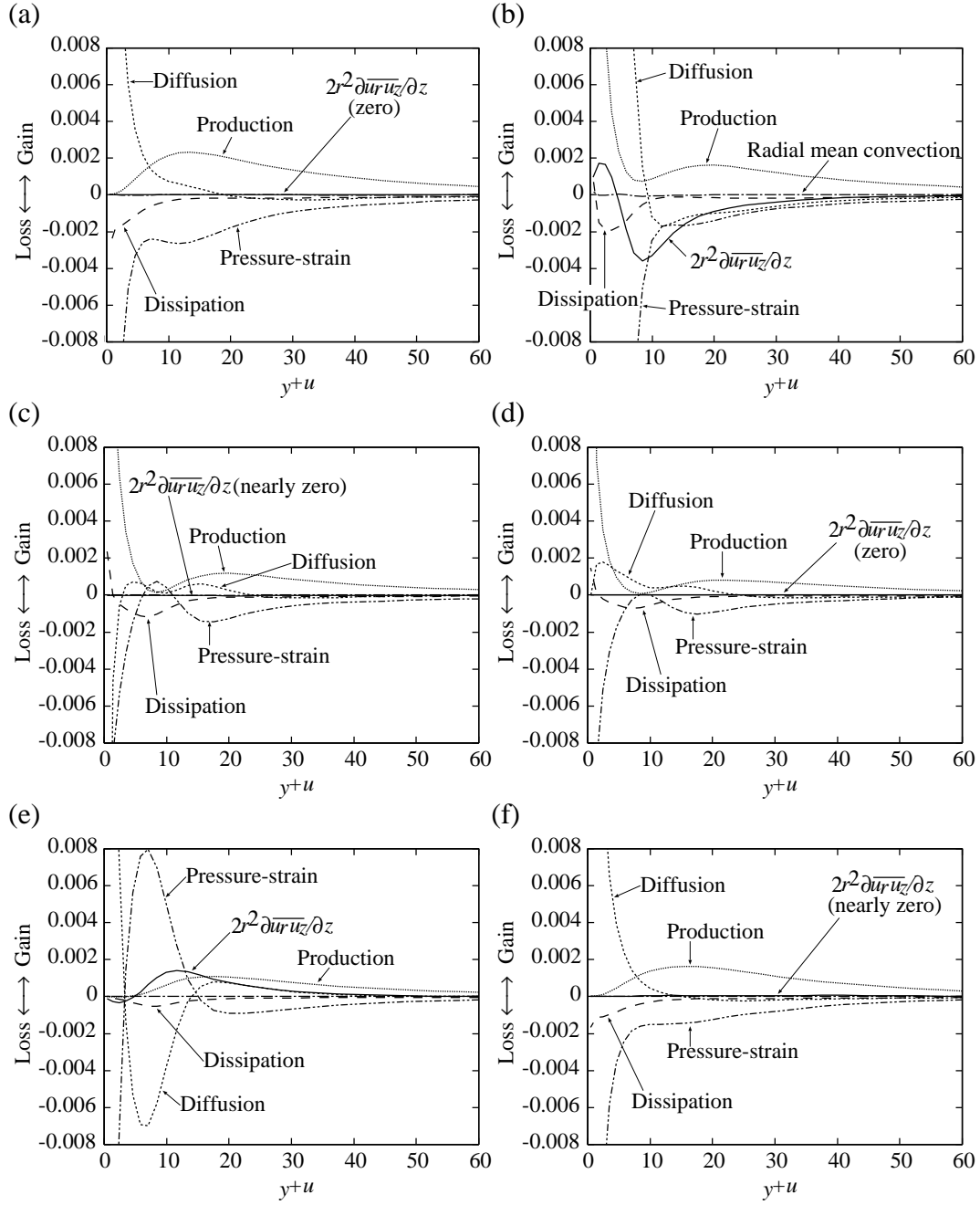
Fig. 10. Budget on the rate-of-change of the weighted Reynolds shear stress, \partial(2r^2u'_x u'_x)/\partial z (Case 4, L_c^{+u} = 7360 , y_d^{+u} = 15 ): (a) steady uncontrolled region ( z^{+u} \simeq -1000 ); (b) rapid drag-reduction region ( z^{+u} \simeq 7 ); (c) gradual drag-reduction region ( z^{+u} \simeq 1000 ); (d) steady controlled region ( z^{+u} - L_c^{+u} \simeq -1000 ); (e) rapid recovery region ( z^{+u} - L_c^{+u} \simeq 7 ); (f) gradual recovery region ( z^{+u} - L_c^{+u} \simeq 1000 ).
