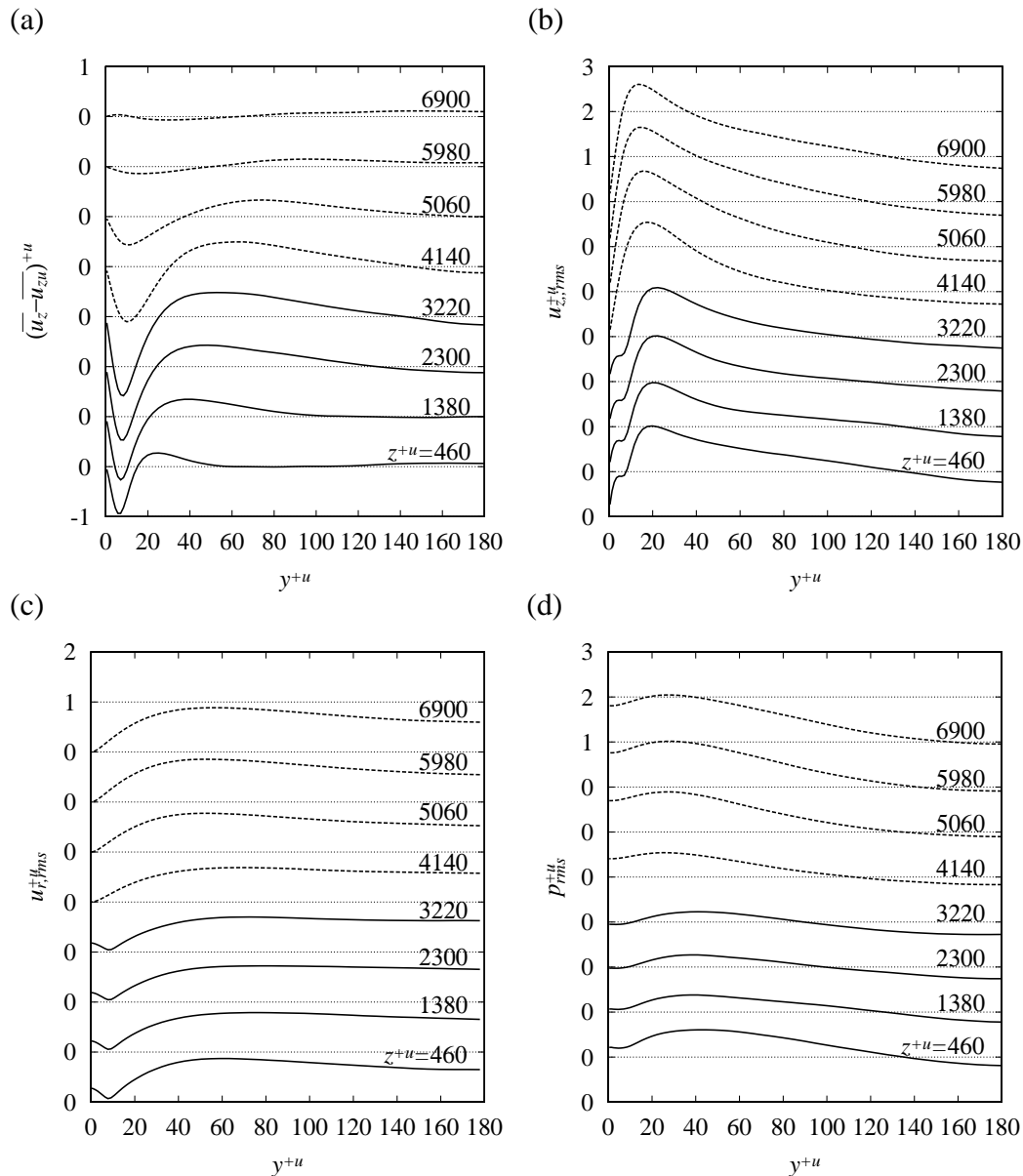
Fig. 7. Flow statistics (Case 3 with L_z^+ = 3680 and y_d^+ = 15 ): (a) deviation of mean velocity from uncontrolled flow; (b) rms longitudinal velocity fluctuation; (c) rms radial velocity fluctuation; (d) rms pressure fluctuation. Solid lines, controlled region; dashed lines, uncontrolled region.
