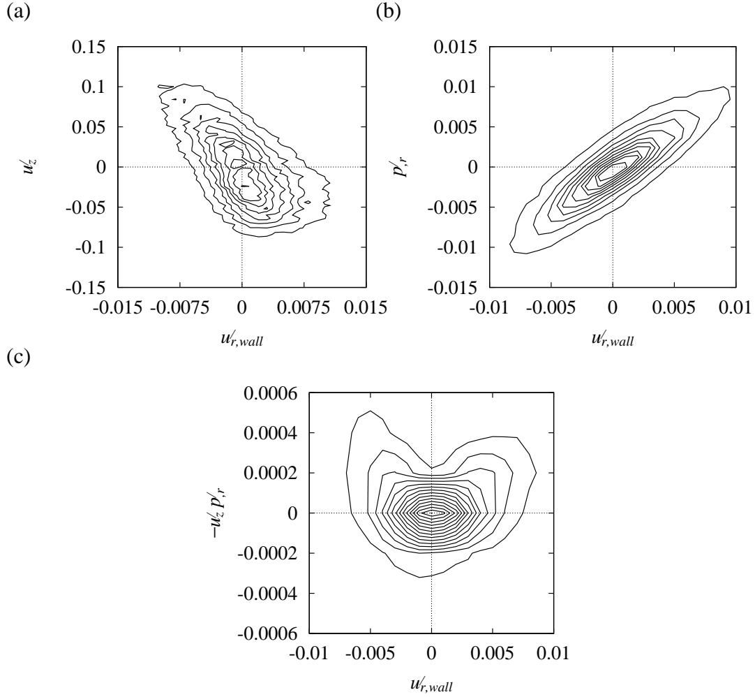
Fig. 12. Correlations between terminal control input, u_{r,wall} ( z^{+u} \simeq L_c^{+u} - 7 ) and quantities right downstream ( y^{+u} \simeq 10 , z^{+u} \simeq L_c^{+u} + 7 ), displayed as isocontours of the probability density function: (a) streamwise velocity fluctuation, u'_z ; (b) fluctuating pressure gradient, p'_{,r} ; (c) the first term in Eq. (17), i.e., -u'_z p'_{,r} .
