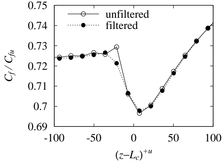
Fig. 6. Effects of the low-pass filter on the local skin friction coefficient (Case 4, L_c^{+u} = 7360 , y_d^{+u} = 15 ).
